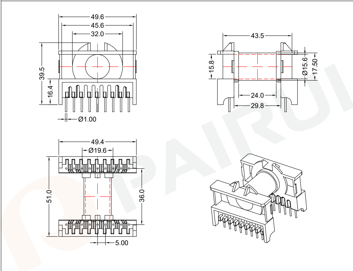
Winding data and area product for 18-pins ETD44/22/15 coil former
