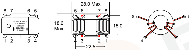
Top view
