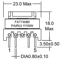
Orthographic view
