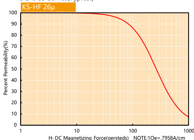
DC-Bias Curves(Typical)
