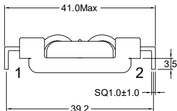
Orthographic view
