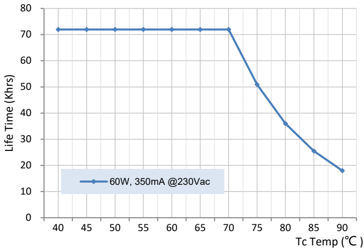
Life Time vs Tc Temp
